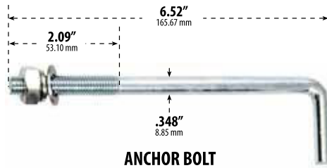
ANCHOR BOLT
