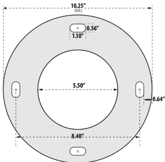
BASE PATTERN
