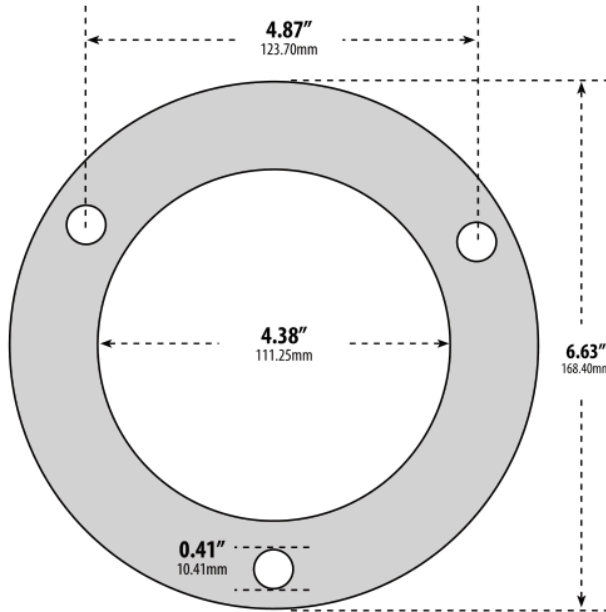
BASE PATTERN
