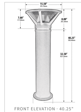
FRONT ELEVATION · 40.25"
