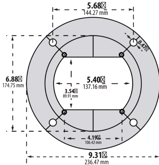
BASE PATTERN
